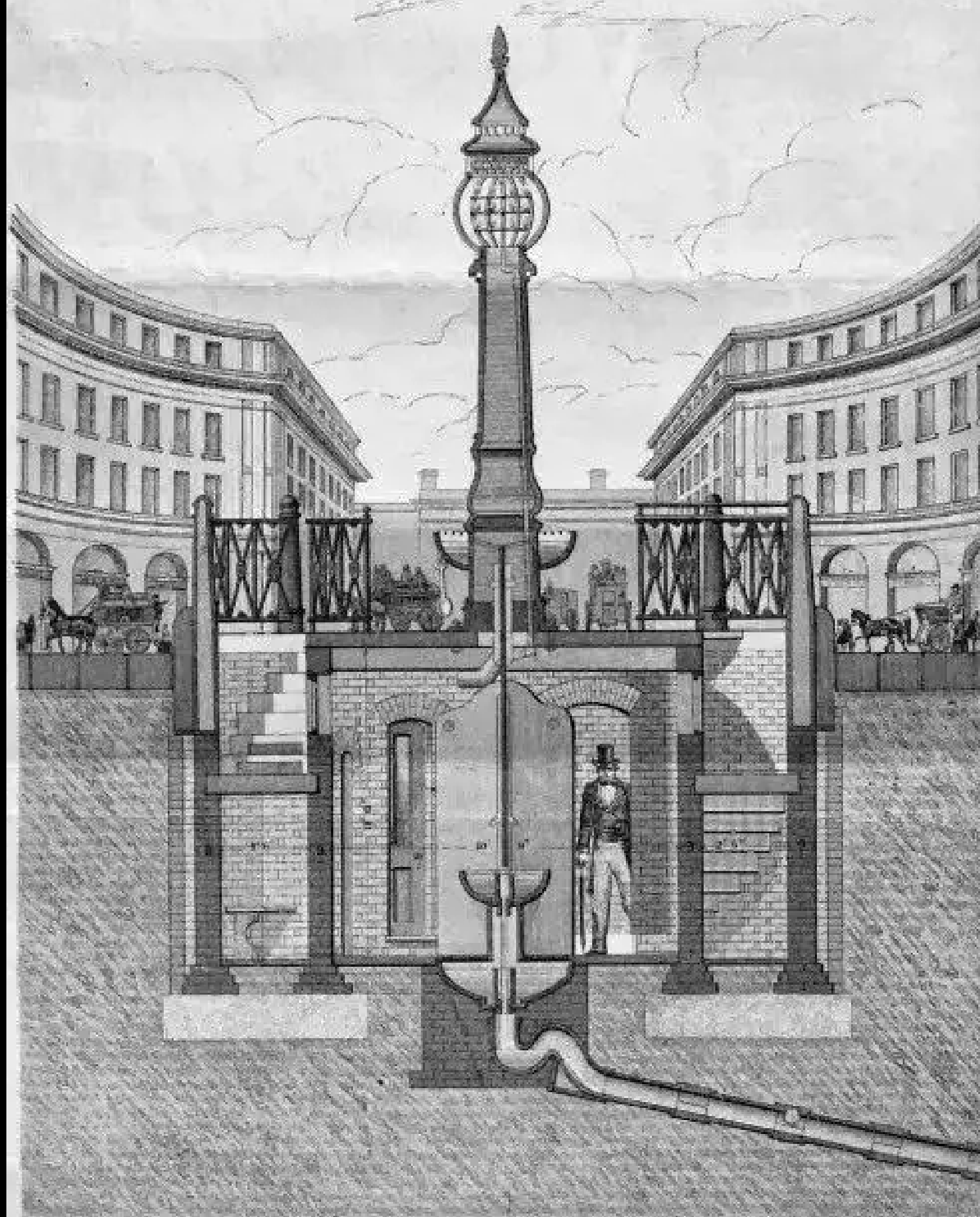
DRAWING SHEWING METHOD OF CONSTRUCTING PUBLIC CONVENIENCES 知乎 @叔兰天际游在东欧 IN A MANNER TO OBVIATE OBJECTIONS TO THEIR APPEARANCE.
